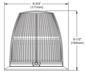
Aerodynamic Dome
